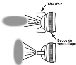
(Plan TP2053)
